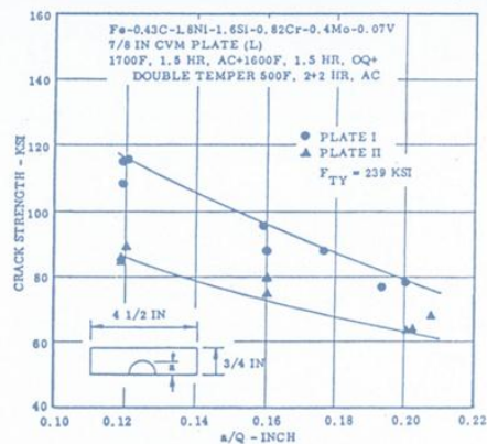
FIG. 3.027124 EFFECT OF SURFACE CRACK SIZE ON CRACK STRENGTH OF CVM PLATE ( F_{TU} = 239 KSI). (16, p. 170)
